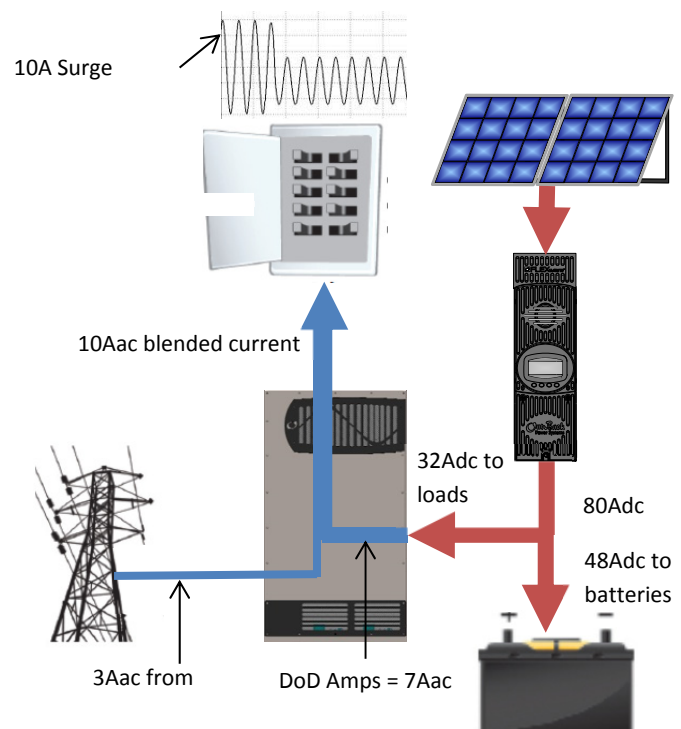
Figure 5 - Grid Zero Current Paths
